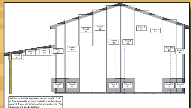
STEEL PANEL LAYOUTS
