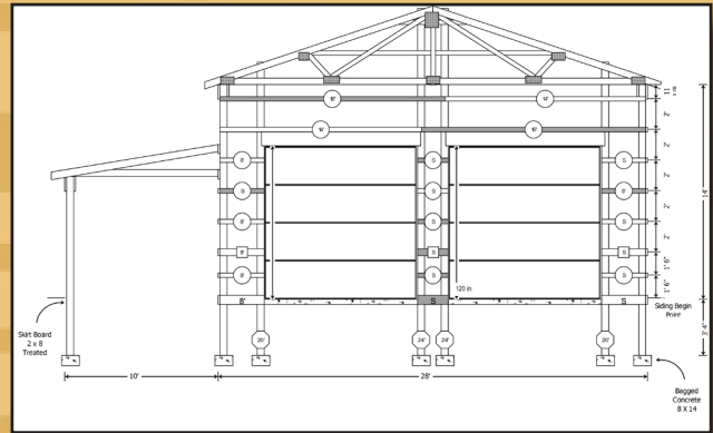
WALL GIRT LAYOUTS
