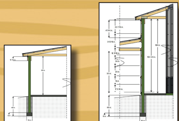
CROSS SECTION DETAILS
